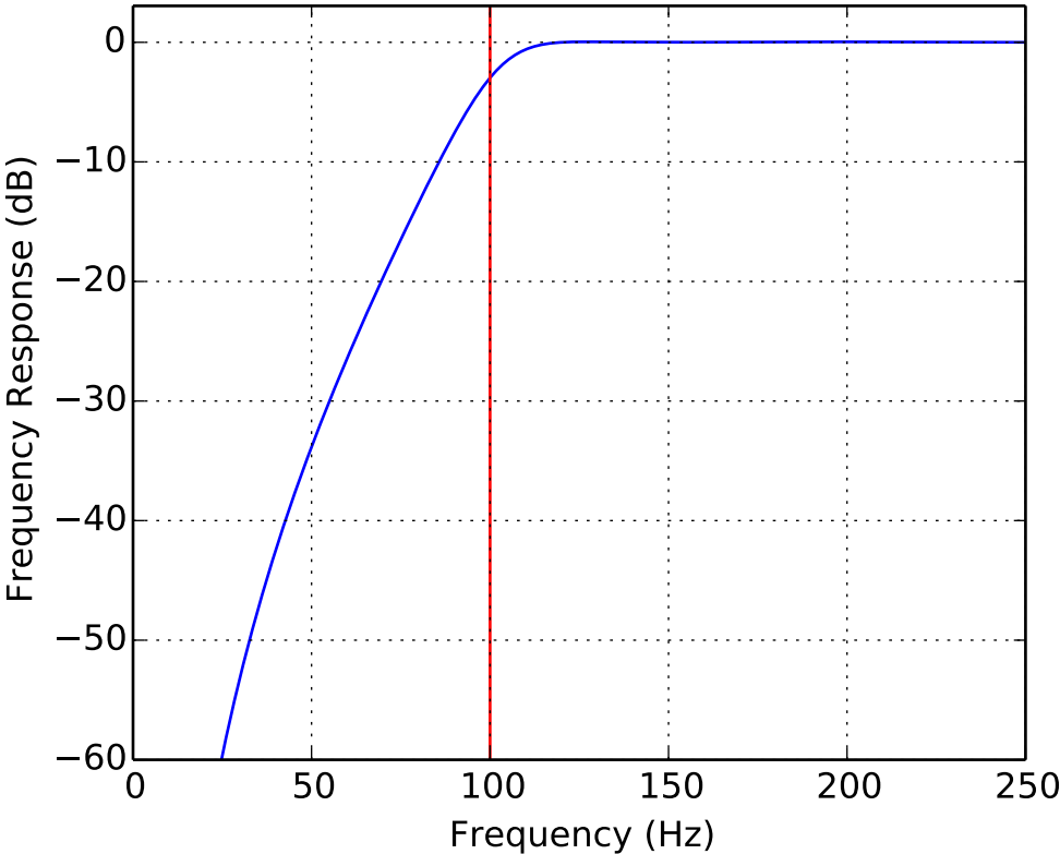
High Pass IIR Frequency Response order = 3, fc = 100.0 Hz, sr = 500.0 Hz
