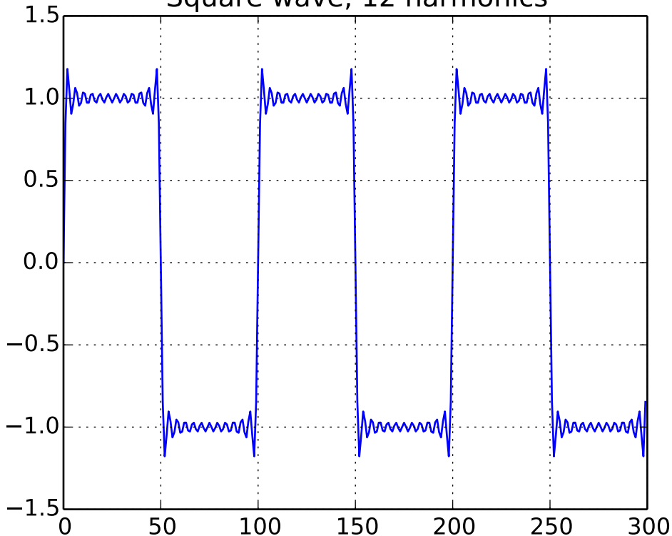
Square wave, 12 harmonics
