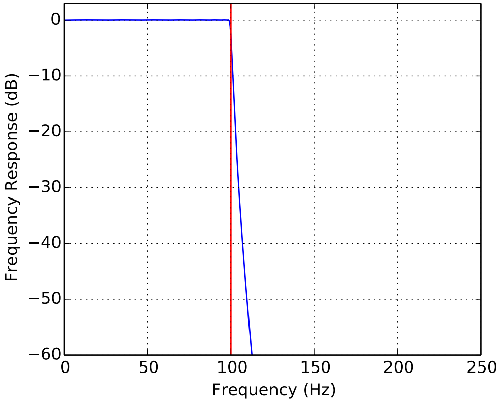
Low Pass IIR Frequency Response order = 15, fc = 100.0 Hz, sr = 500.0 Hz
