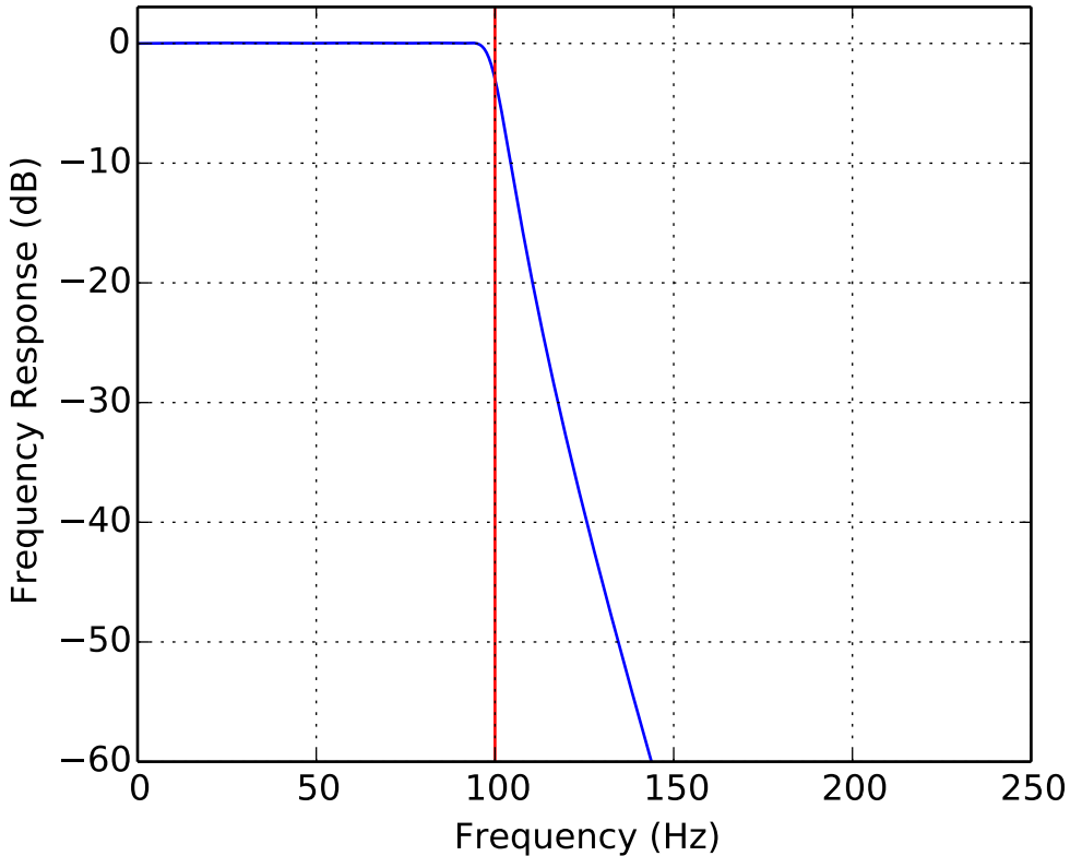
Low Pass IIR Frequency Response order = 7, f_c = 100.0 Hz, sr = 500.0 Hz
