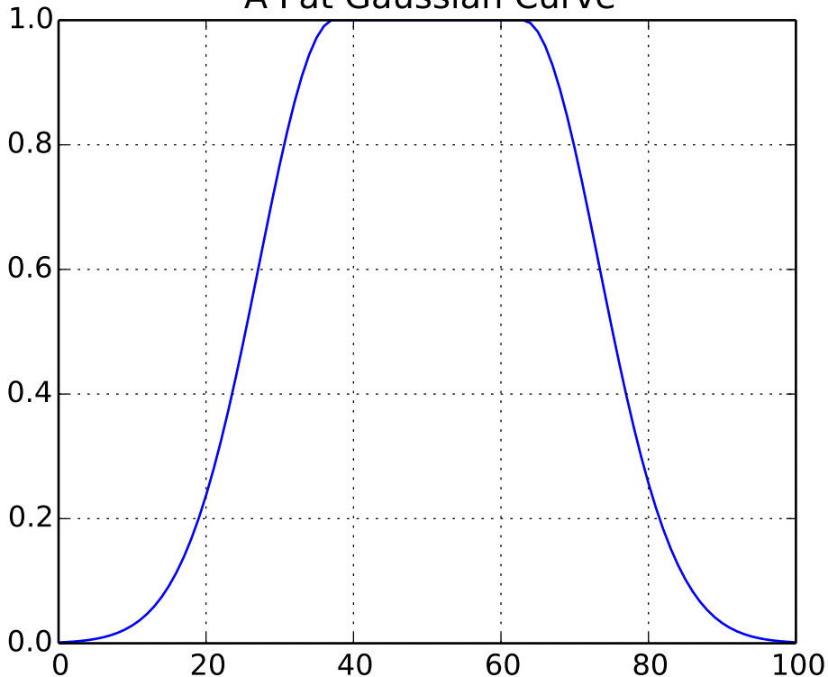
A Fat Gaussian Curve
