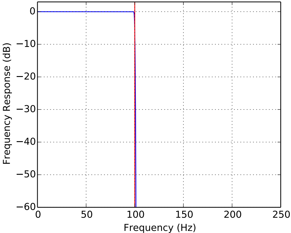
Low Pass FIR Frequency Response order = 1024, fc = 100.0 Hz, sr = 500.0 Hz
