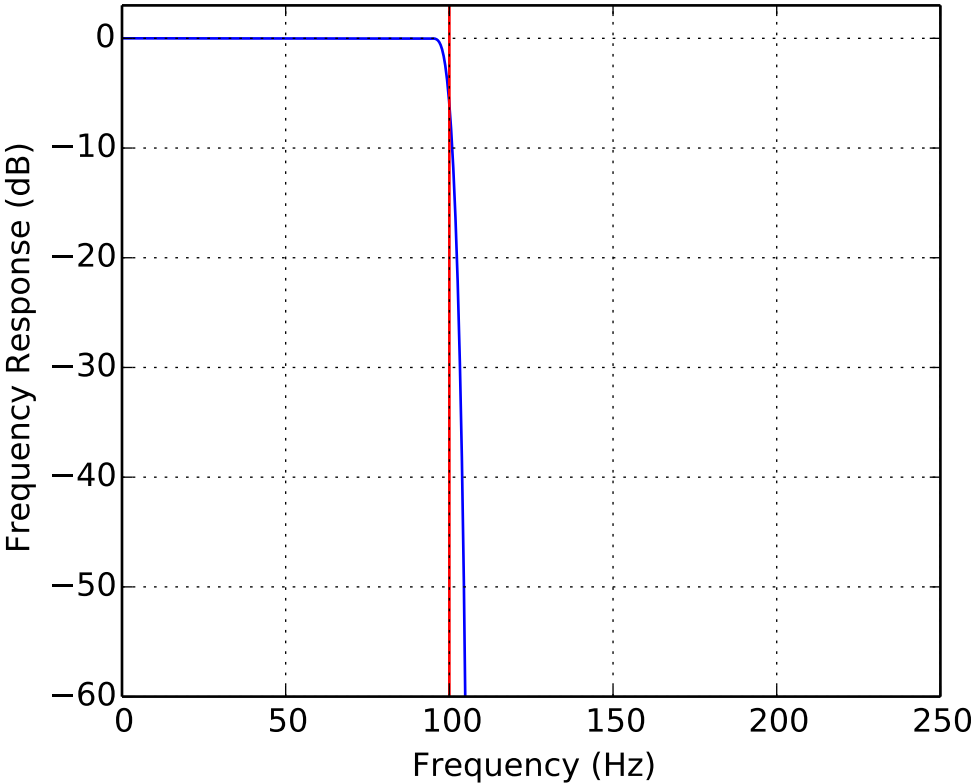
Low Pass FIR Frequency Response order = 256, fc = 100.0 Hz, sr = 500.0 Hz
