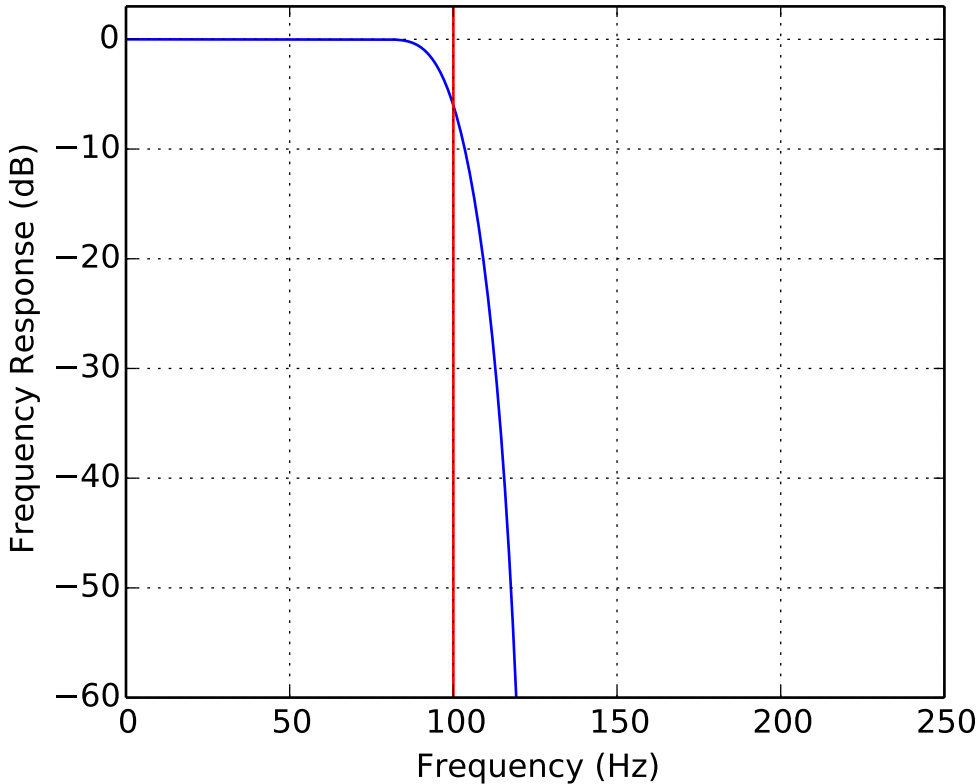
Low Pass FIR Frequency Response order = 64, f_c = 100.0 Hz, sr = 500.0 Hz
