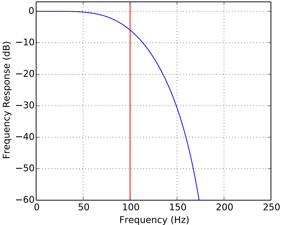
Low Pass FIR Frequency Response order = 16, fc = 100.0 Hz, sr = 500.0 Hz
