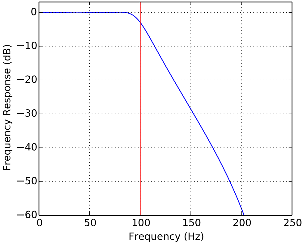
Low Pass IIR Frequency Response order = 3, fc = 100.0 Hz, sr = 500.0 Hz
